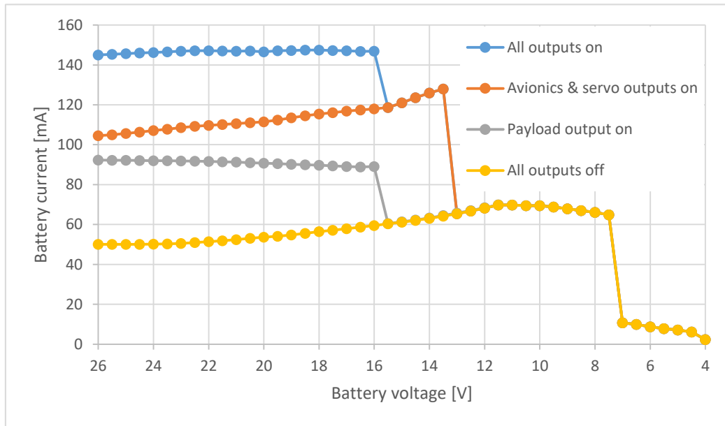
Graph 2 – Quiescent battery current
