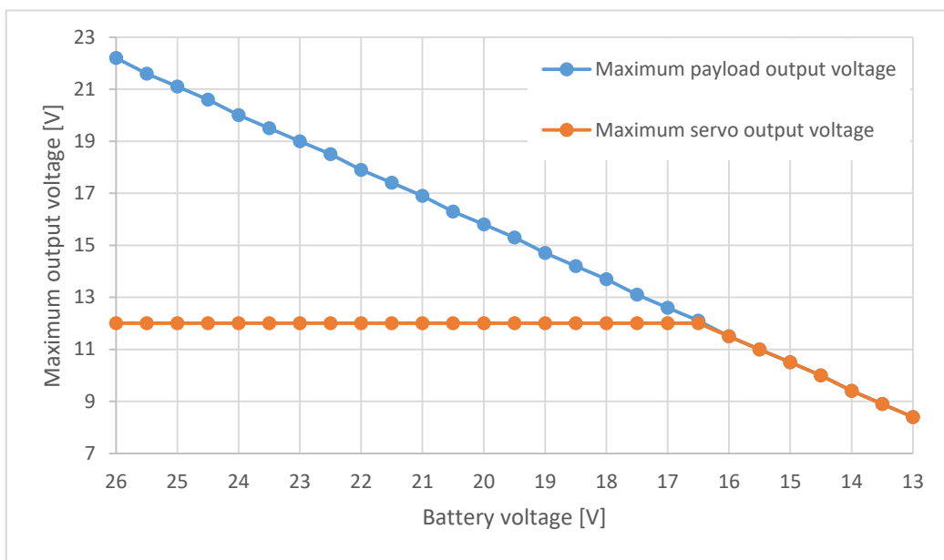
Graph 4 – Maximum payload and servo output voltages
