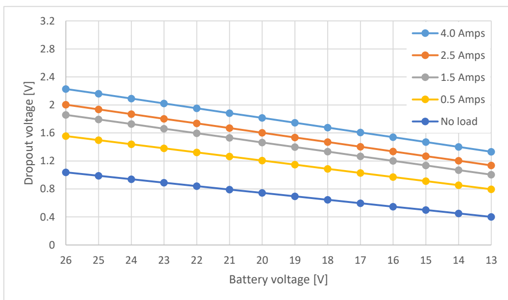
Graph 3 – Avionics output dropout voltage
