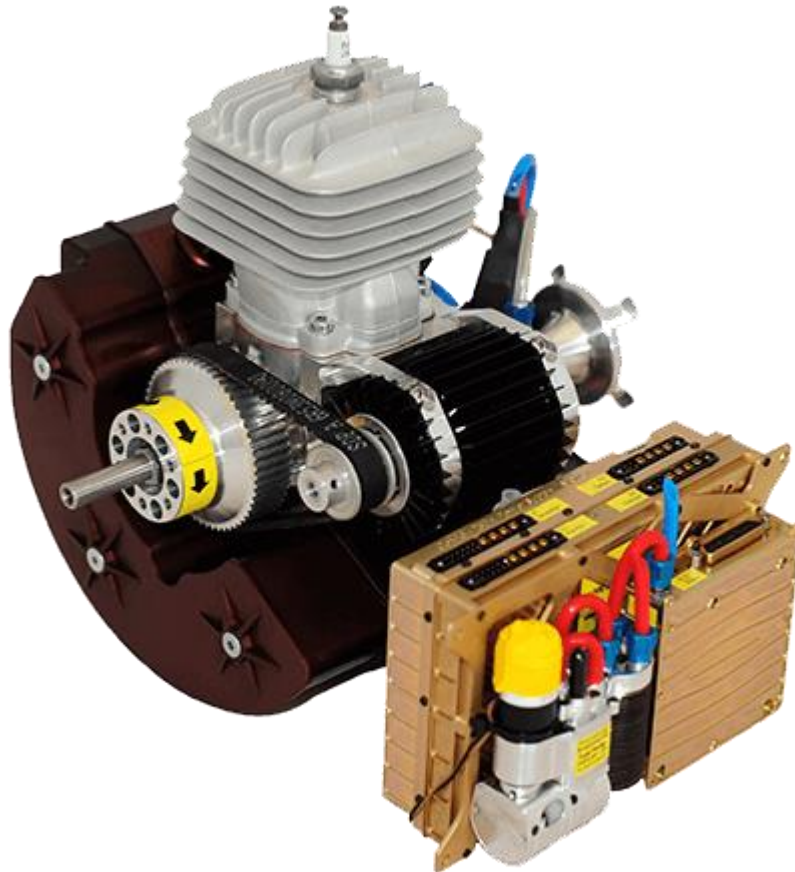
Figure 4 –Corvid 29 engine package from Currawong Engineering
